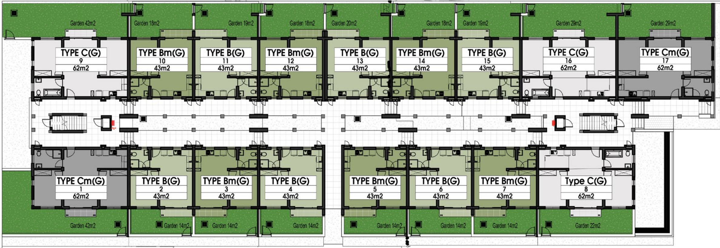
GROUND FLOOR
