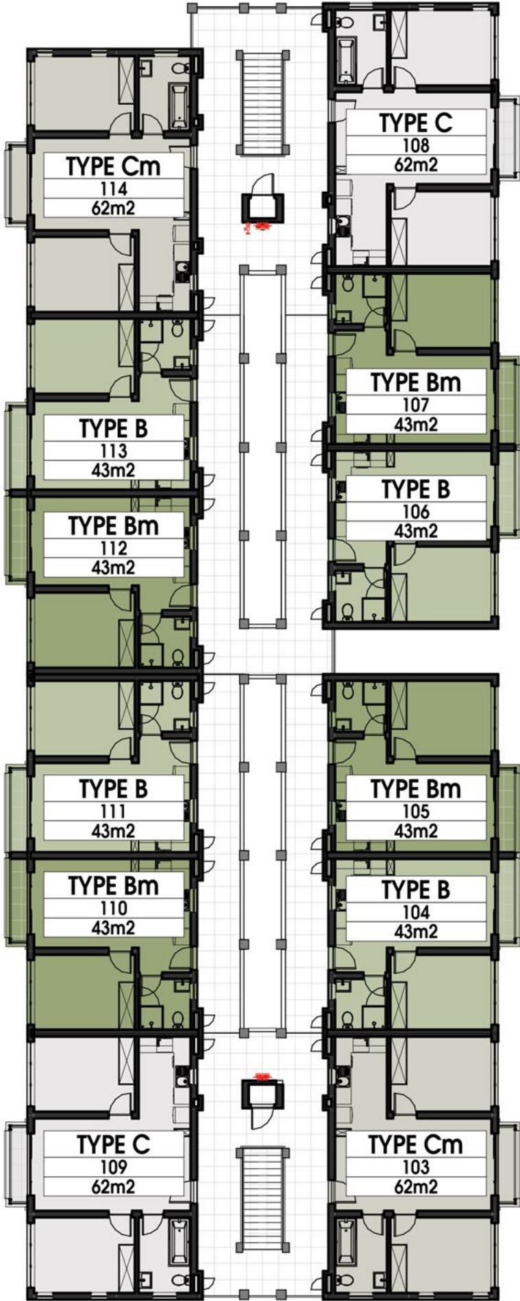
THIRD FLOOR
