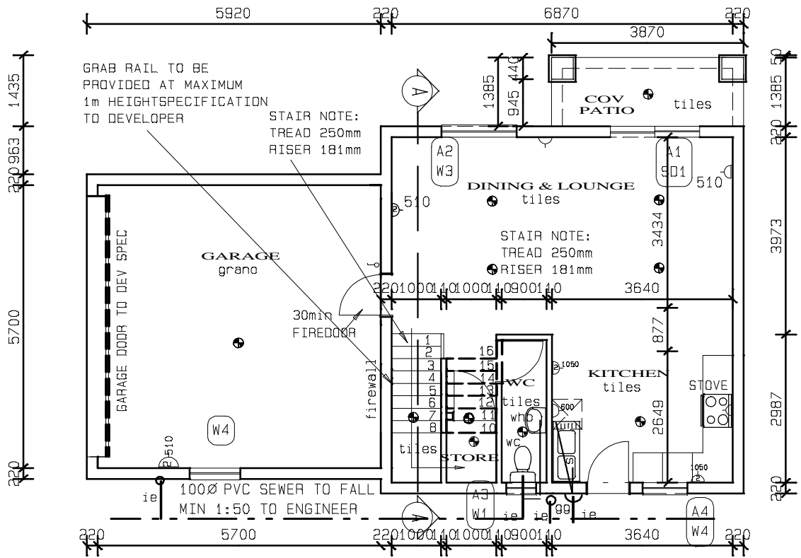
GROUND FLOOR STOREY SCALE 1:100
