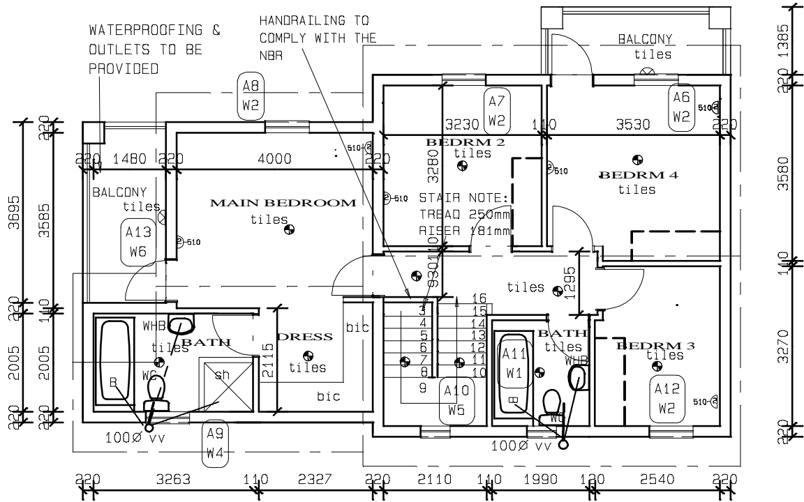
FIRST FLOOR STOREY SCALE 1:100
