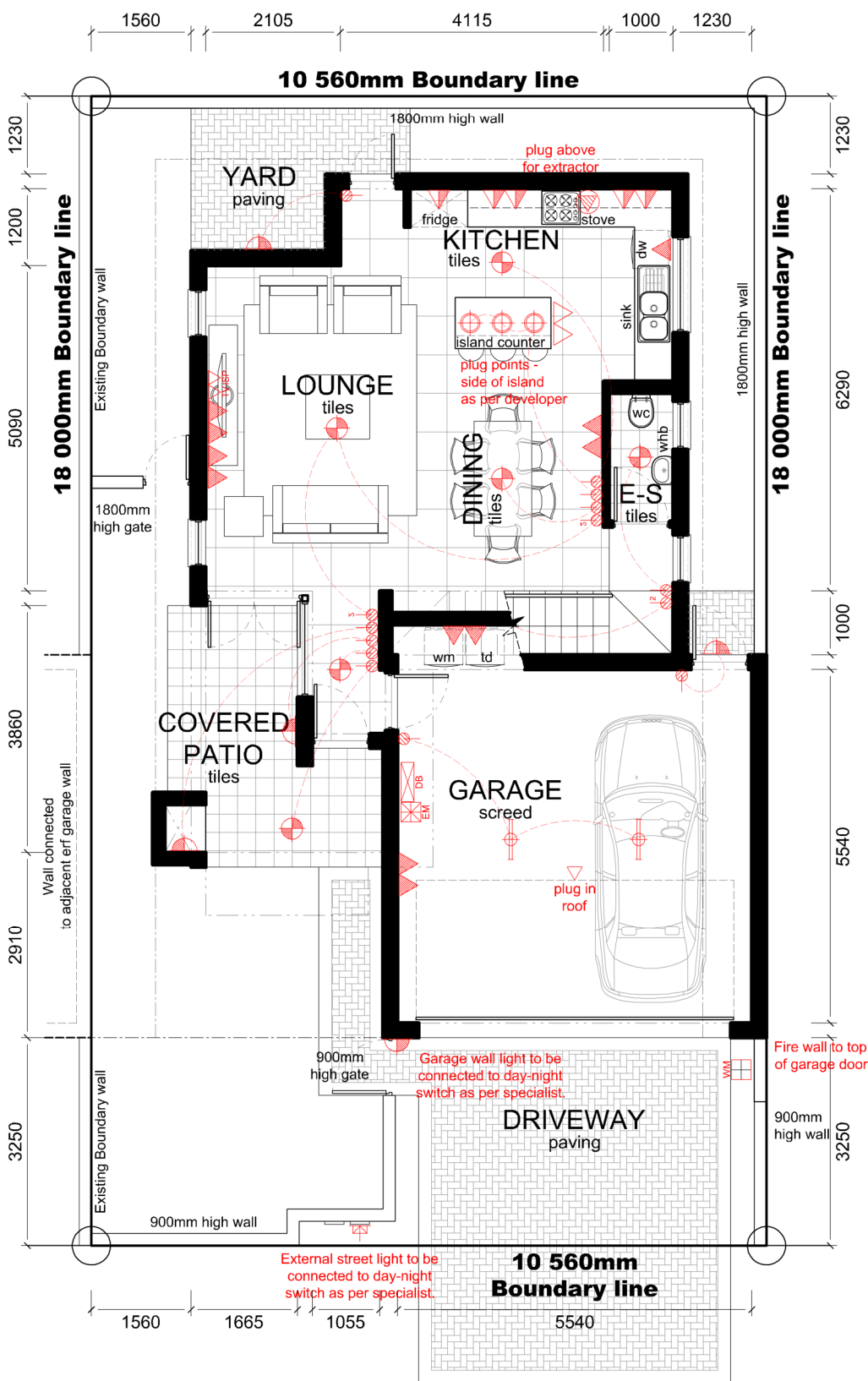
MEADOW CIRCLE GROUND STOREY PLAN
