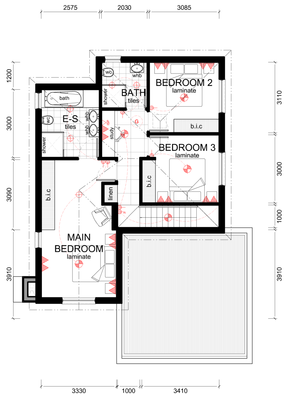
FIRST STOREY PLAN
