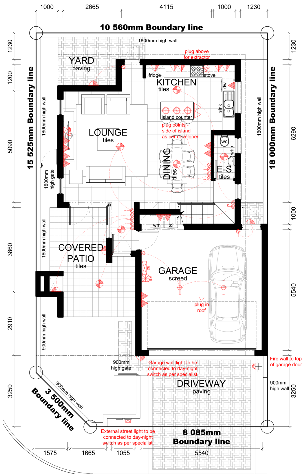
MEADOW CIRCLE GROUND STOREY PLAN
