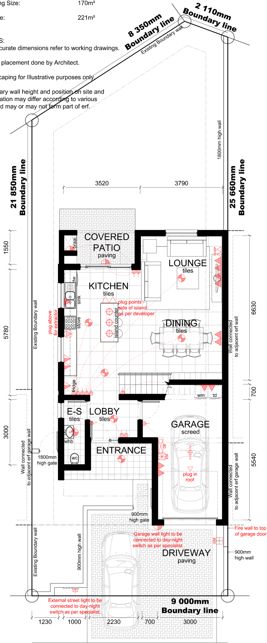
GROUND STOREY PLAN
