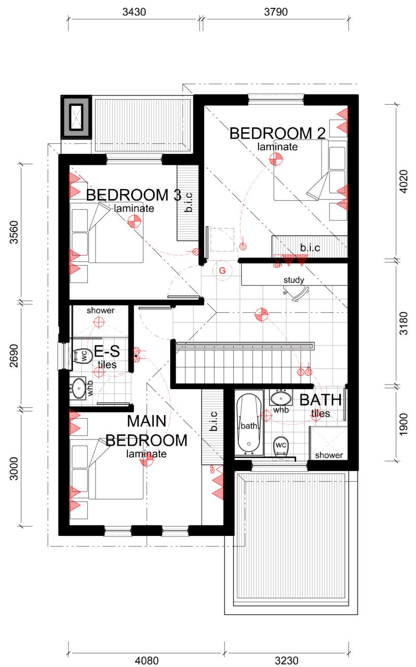
FIRST STOREY PLAN
