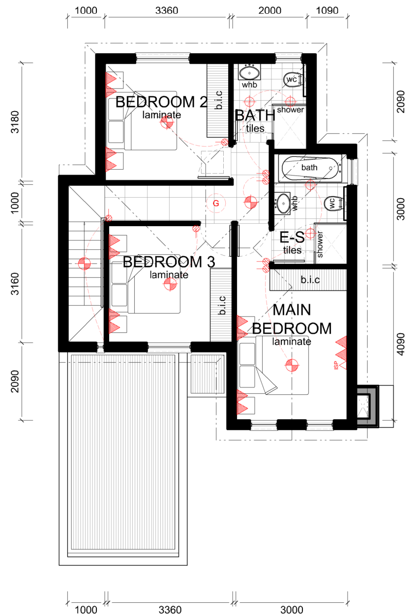
FIRST STOREY PLAN
