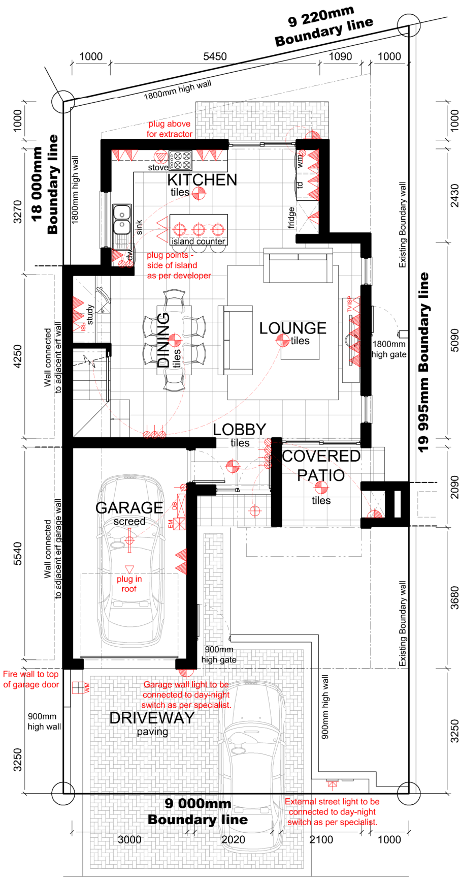
GROUND STOREY PLAN
