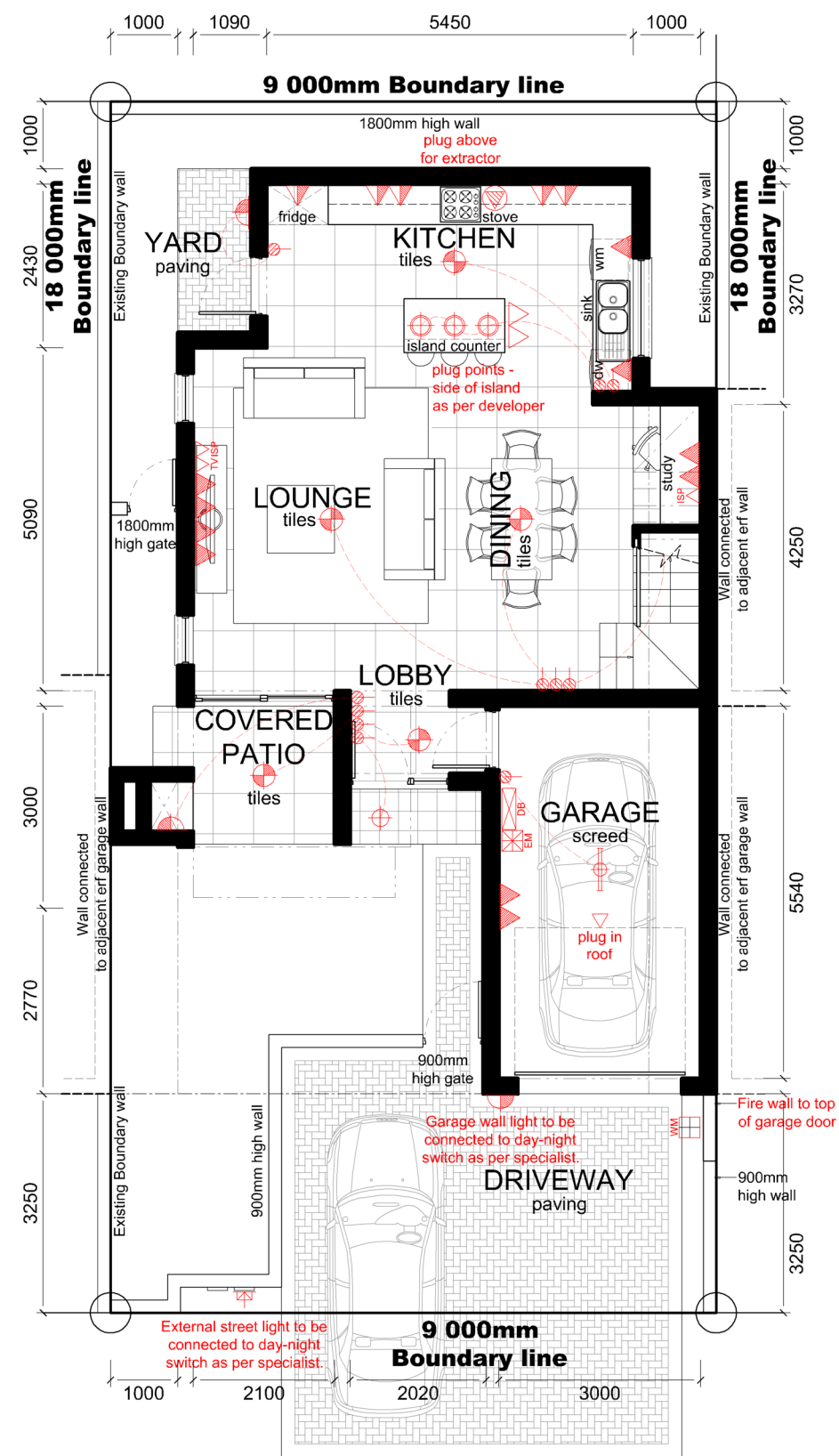
GROUND STOREY PLAN
