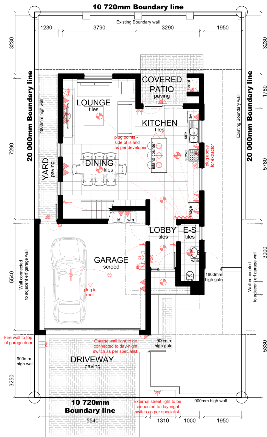
HARVEST CRESCENT GROUND STOREY PLAN
