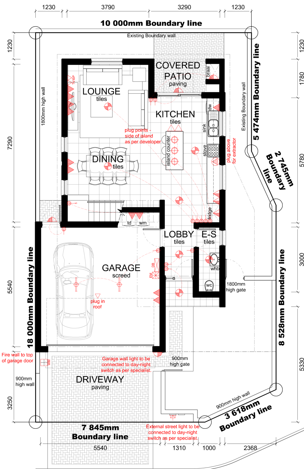
MAIZE LANE GROUND STOREY PLAN
