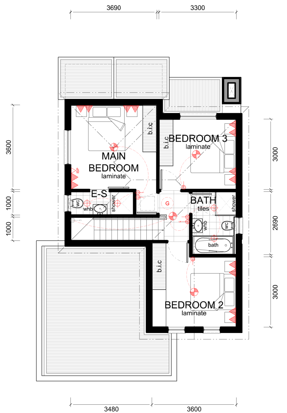
FIRST STOREY PLAN
