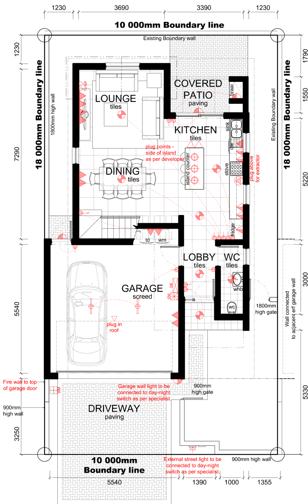
MAIZE LANE GROUND STOREY PLAN
