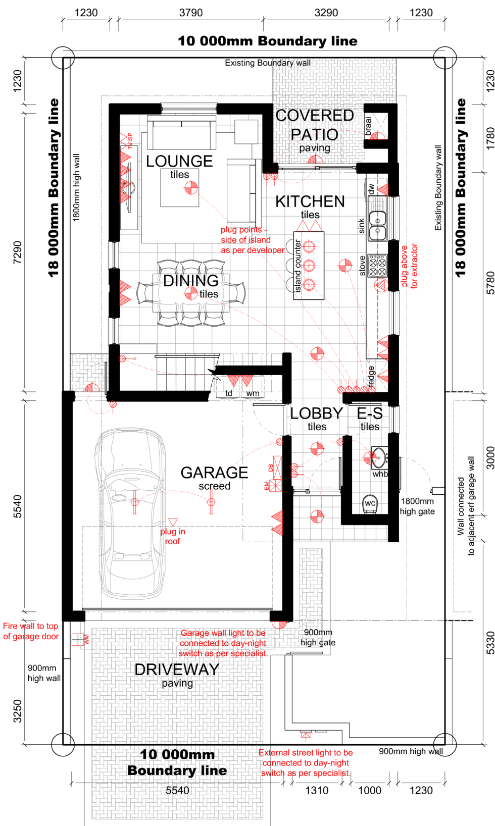
MAIZE LANE GROUND STOREY PLAN
