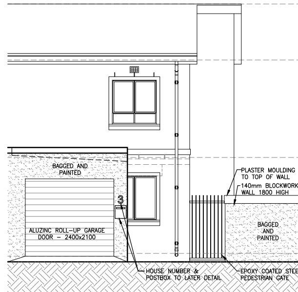
FRONT STREET ELEVATION
