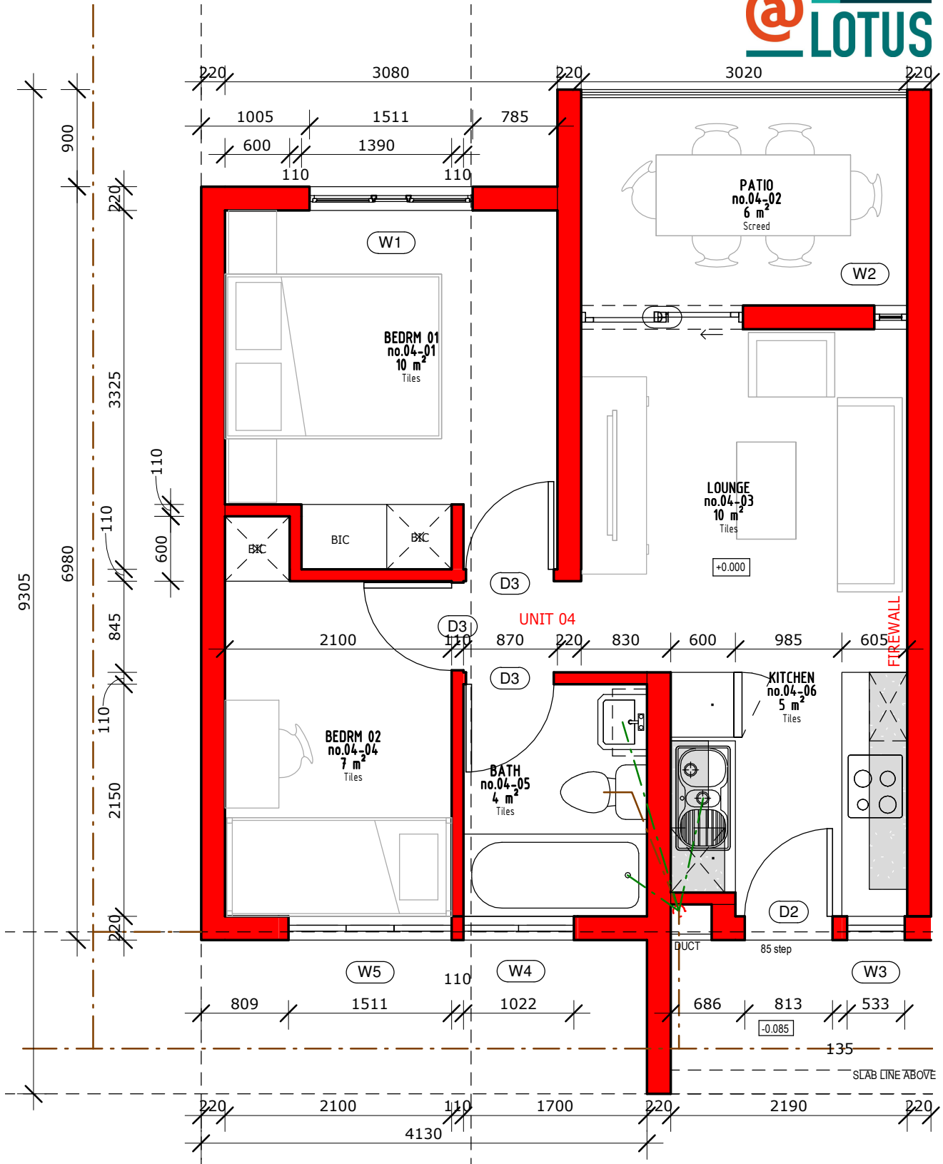
TYPICAL UNIT LAYOUT SCALE 1 : 50
