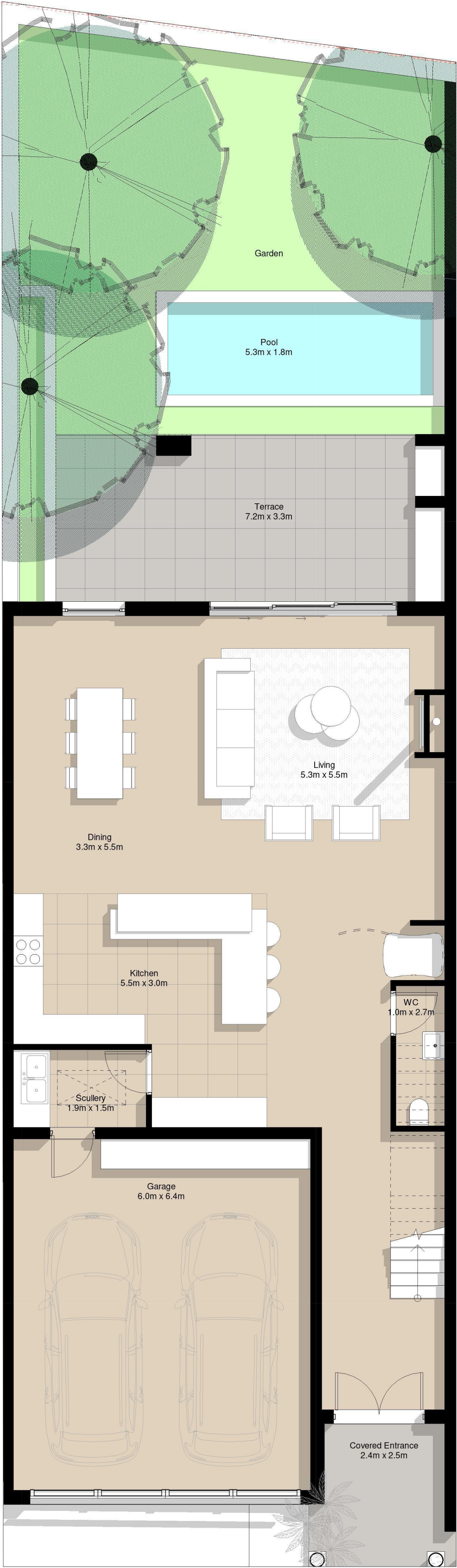
Ground Floor
